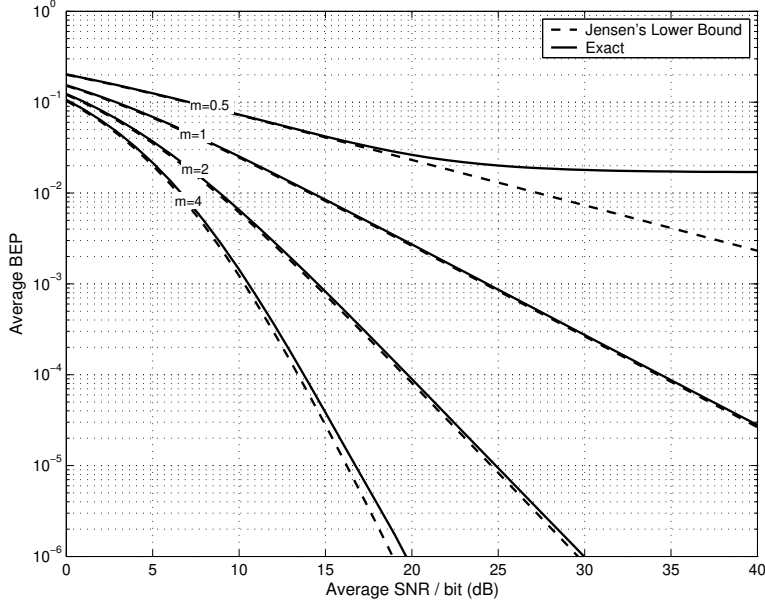
Figure 2.1. Average bit error probability of partially coherent Nakagami- m BPSK channel, \sigma_\epsilon = 16^\circ . This is just additional wording to make this caption stretch to another line..
